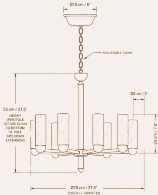
FRONT ELEVATION SCALE 1:5
